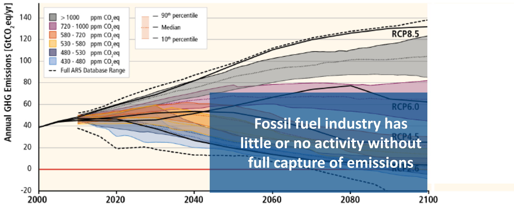
GHG Emission Pathways 2000-2100: All AR5 Scenarios
