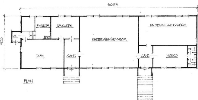
Plantegning.
