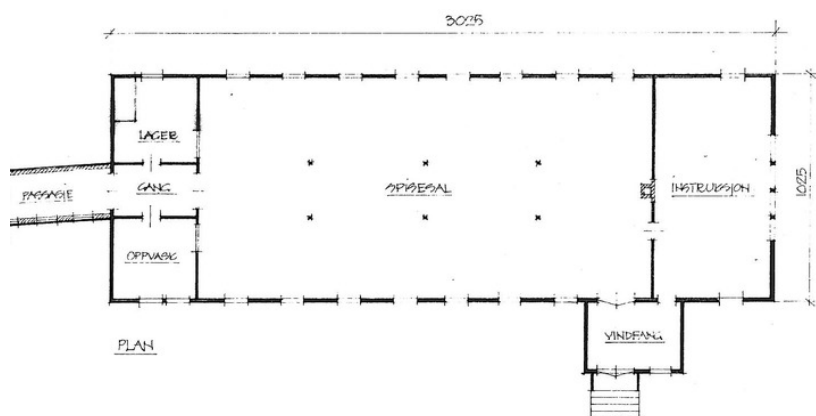
Plantegning.
