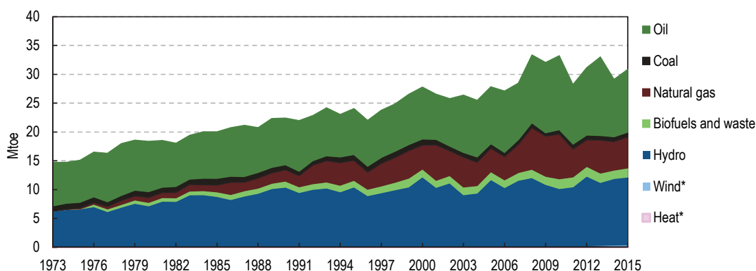
Figure 1.3 TPES, 1973-2015
